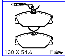
PL23554-1 THK 16.2
