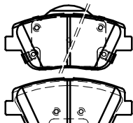
132.8 X 58.9 F
