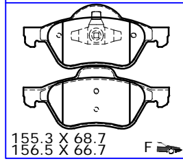
PL24065 THK 17.8
