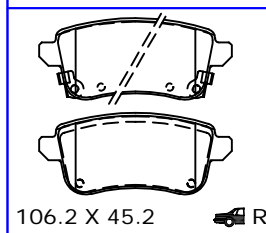
PL80192 THK 15.5
