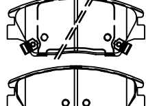
PL22590 THK 17.7
