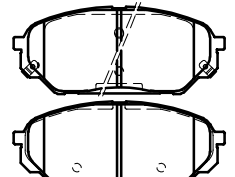
155 X 64.3 F
