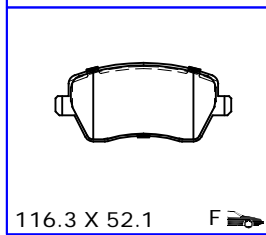
PL25702 THK 17.5
