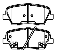
116.8 X 48.7 R
