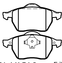
PL21911 THK 19.6
