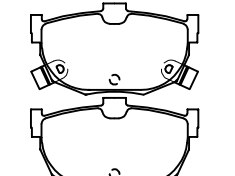
85.2 X 46.4 R
