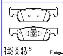
PL80192 THK 15.5
