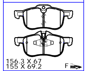
PL80147 THK 18.8
