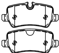
PL80184 THK 16.5
