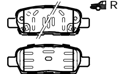
PL23871 THK 14.4
