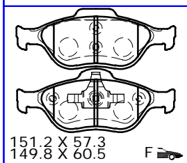
PL22525 THK 17
