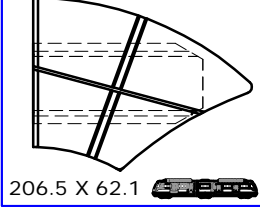
PL70046-2 THK 24
